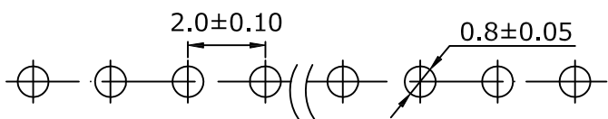
RECOMMENDED PCB LAYOUT
