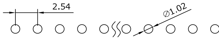
Recommended PCB Layout (PCB TOLERANCE ±0.05)
