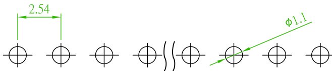
Recommended PCB Layout (PCB TOLERANCE ±0.1)
