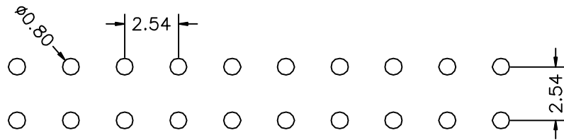
PCB LAYOUT
